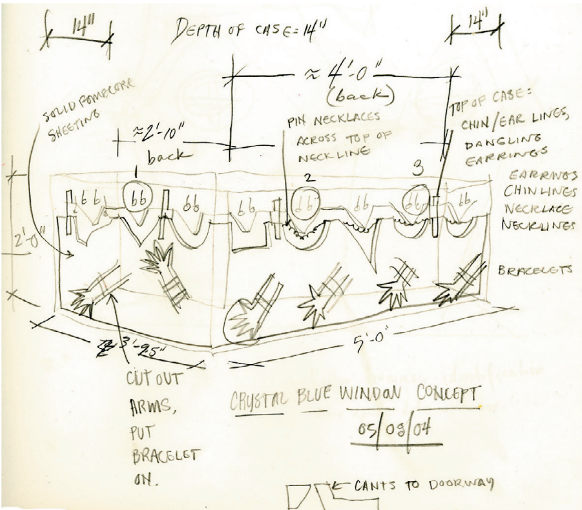
Crystal Blue Beading, window armature for beaded jewelry display.
